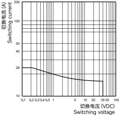
允许最大负载范围 (23°C) Max.imum allowable load range
